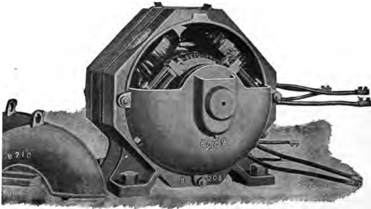
FIG. 206.—The "Lundell" Octagon Four-pole Motor, with case open, showing parts. Laminated field magnets and armature core. For vehicle use ranging between 2.5 and 15 horse power, wound for 80 volts. At this pressure the 2.5 horse power takes 28.5 amperes; the 5 horse power, 55 amperes; the 10 horse power, 110 amperes; the 15 horse power, 160 amperes.
